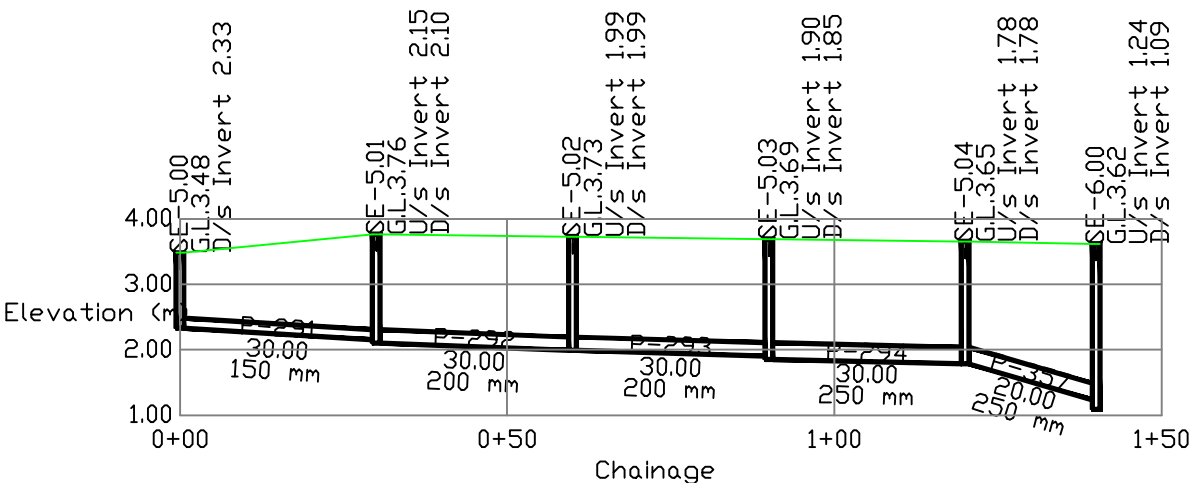
Profile: TA-5 TO OUTFALL
