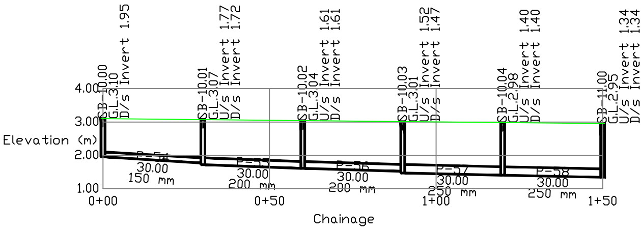
Profile: SB-10 TO SB-11.0
