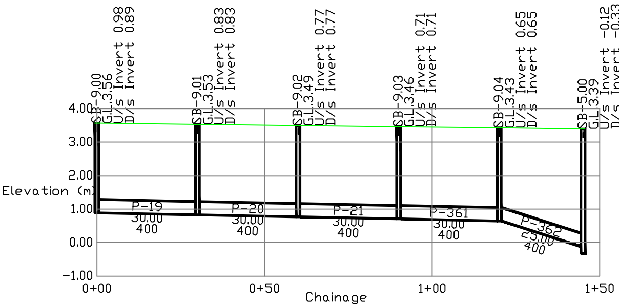
Profile: SB-9 TO SB-5
