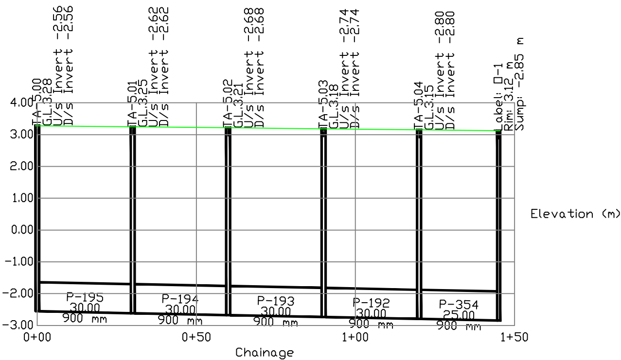
Profile: TA-5 TO OUTFALL
