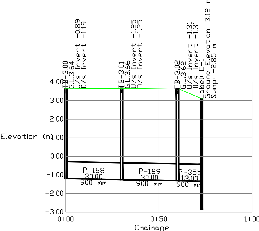
Profile: TB-3.0 TO □ □-1
