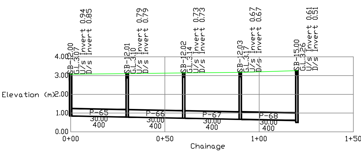
Profile: SB-12 TO SB-15
