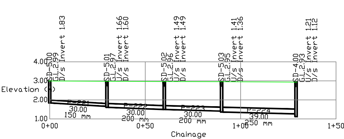
Profile: SD-5 TO SD-4
