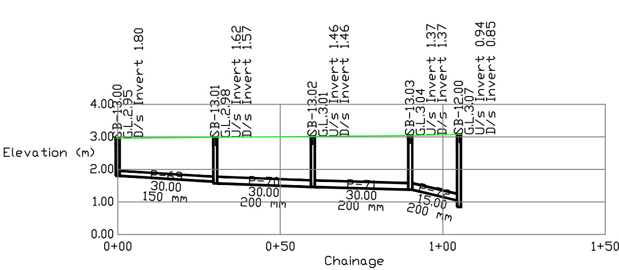
Profile: SB-13 TO SB-12
